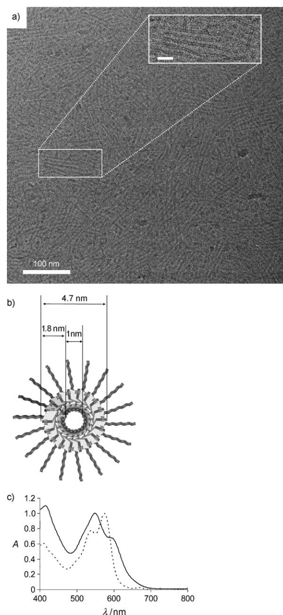
Figure 2. a) Cryo-TEM image of a solution of 2 ( 2 \times 10^{-4} M) in water/THF (9:1 v/v). The inset shows an enlarged image of a nanotube (scale bar 20 nm). b) Suggested structure of the nanotubes (nanotube cross section; see Figure S13 in the Supporting Information for an enlargement of image (a)). c) Normalized UV/Vis spectra of a solution of 2 in dichloromethane (disassembled, dotted line) and in water/THF (9:1 v/v) solution (solid line).
